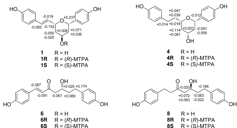
Figure 2. \Delta\delta_{S-R} values of MTPA esters of 1 , 4 , 6 , and 8 used for the determination of absolute configuration.
