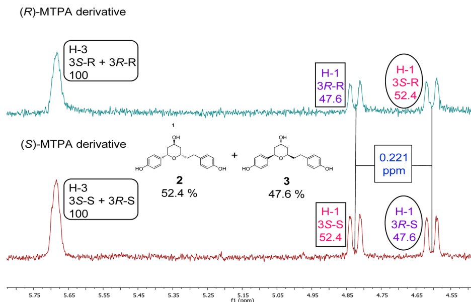
Figure 3. Comparison of the ^1\text{H} NMR spectra of the MTPA esters of the enantiomeric mixture of 2 and 3 ( \delta_{\text{H}} 4.5 to 5.8). The resonances of H-1 and H-3 could be readily assigned on the basis of their chemical shifts and splitting patterns. However, the four resonances of H-1 revealed a small but significant difference in their integrals (47.6:52.4, and vice versa), providing evidence for the fact that the isolate was an enantiomeric mixture of 2 and 3 rather than a pure single enantiomer.
