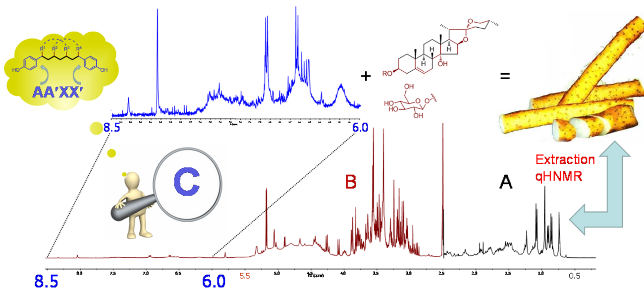
Figure 1. Representation of the concept of ^1\text{H} NMR-guided fractionation for the metabolomic mining of Dioscorea phytoconstituents. A 30 mg aliquot of crude MeOH extract of wild yam was carefully dried in vacuo and dissolved in 600 \mu\text{L} of \text{DMSO}-d_6 , and a high S/N ^1\text{H} NMR spectrum was collected (400 MHz, 5 mm broadband probe with ATM, NS = 5 K). Under these conditions, signals in the aromatic region between \delta_{\text{H}} 6.0 and 8.5 (2.47%) were readily detected, and some of them could even be recognized as diagnostic AA'XX' resonances of the subsequently isolated diarylheptanoids.
