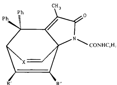
1 X = CH, N, R' = R'' = H or (CH=CH) 2
