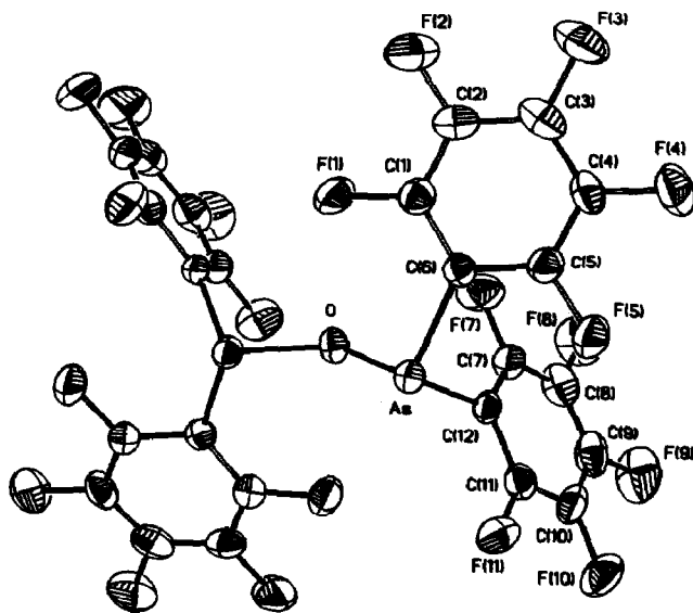
Fig. 4. Molecular structure and numbering scheme for (\text{C}_6\text{F}_5)_2\text{AsOAs}(\text{C}_6\text{F}_5)_2 ( 2 ). A crystallographic two-fold axis contains the oxygen atom and is in the As–O–As(a) plane.
