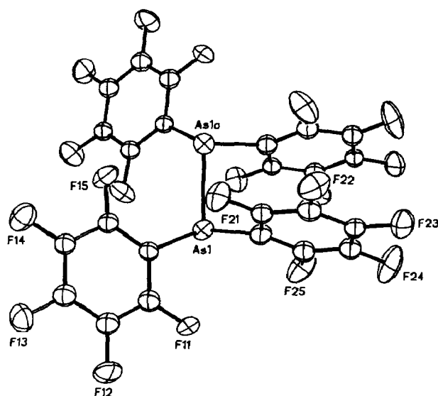
Fig. 1. Molecular structure and numbering scheme for (\text{C}_6\text{F}_5)_2\text{AsAs}(\text{C}_6\text{F}_5)_2 (1); the C and F atoms have the same numbers. One of three crystallographically independent, but chemically similar, molecules is shown. A two-fold axis bisects the As–As(a) bond and lies approximately in the paper plane.
