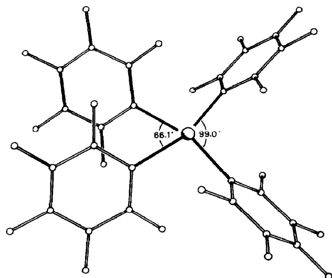
Fig. 3. A view of 1 along the As-As(a) bond with the average C-As-As'-C' torsion angles.
