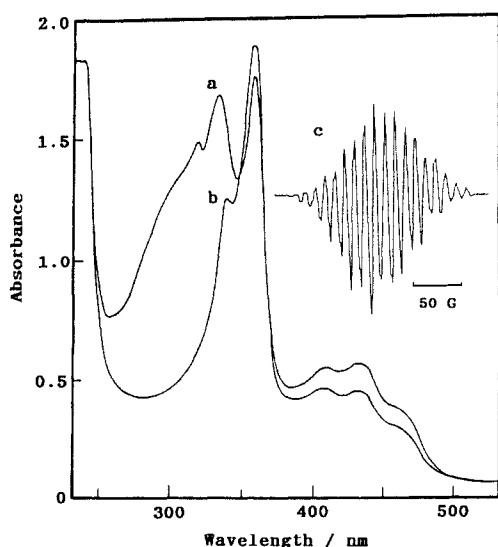
Figure 1. (a) Electronic absorption spectrum observed in the reaction of (\text{AcrH})_2 ( 5.0 \times 10^{-5} M) with \text{Ph}_3\text{C}^+ ( 1.0 \times 10^{-4} M) in deaerated MeCN and (b) that after introducing dioxygen to the solution. (c) ESR spectrum observed in the reaction of (\text{AcrH})_2 ( 1.5 \times 10^{-3} M) with \text{Ph}_3\text{C}^+ ( 1.5 \times 10^{-3} M) in deaerated MeCN.
