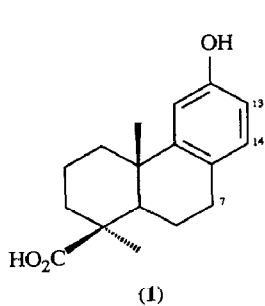
Scheme 1
