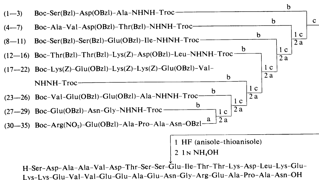
Fig. 2. Synthetic Route to Deacetyl-thymosin \alpha_{11}
