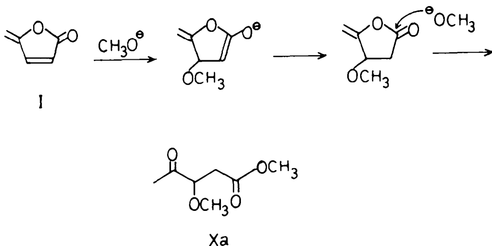
Scheme 5
