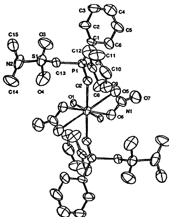
Fig. 2. Molecular structure and atom labeling scheme for \text{UO}_2(\text{NO}_3)_2[(\text{C}_6\text{H}_5)_2\text{P}(\text{O})\text{CH}_2\text{S}(\text{O})_2\text{N}(\text{CH}_3)_2]_2 .
