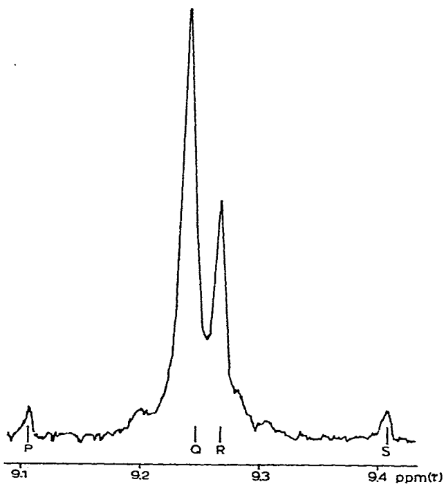
Fig. 2. ^1\text{H} NMR spectrum of the phenyl cage compound (Vb) (aromatic H omitted; solvent, \text{CDCl}_3 ; sweep width, 100 Hz).
