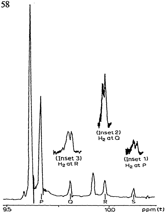
Fig. 1. ^1\text{H} NMR spectrum of the methyl cage compound (Va) (Solvent, benzene; sweep width, 250 Hz).
