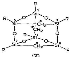
(Va, R = CH 3 ; Vb, R = C 6 H 5 )
