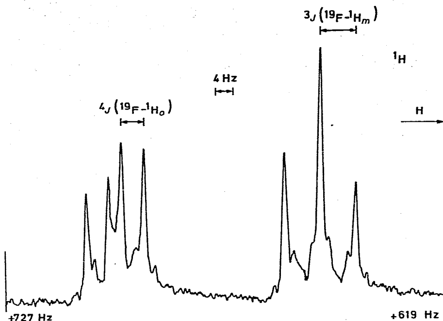
Fig. 2. ^1\text{H} NMR spectrum of (4\text{-FC}_6\text{H}_4)_3\text{AsO} ( \delta in Hz relative to TMS).
