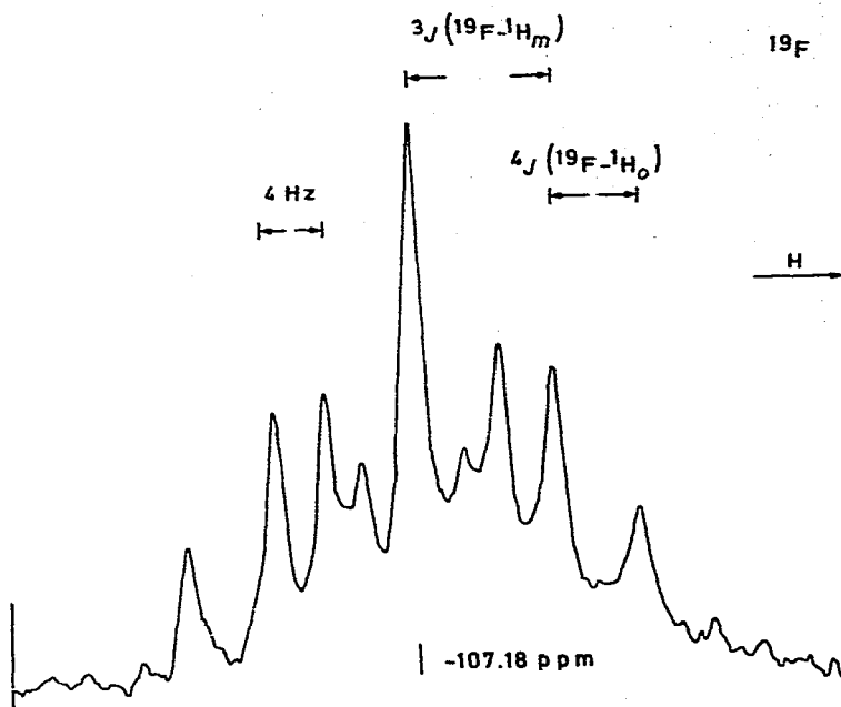
Fig. 4. ^{19}\text{F} NMR spectrum of (4\text{-FC}_6\text{H}_4)_3\text{AsO} ( \delta in ppm relative to \text{CCl}_3\text{F} ).
