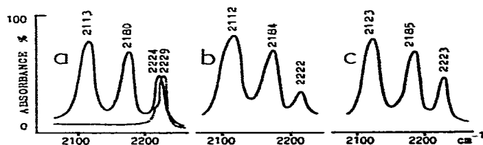
Fig. 1. IR spectra of: (a) (.....) compound 29, 0.03 M in DMSO; (—) its dimeric dianion, electrochemically generated in DMSO. (b) Dimeric dianion of compound 29, prepared by reduction with naphthalene-potassium in DME. (c) Sodium methoxide adduct of the same compound, 0.03 M in DMSO. Band assignment: 2229 \text{cm}^{-1} , superposition of the three types \nu(\text{CN}) ; 2112–2123 \text{cm}^{-1} , \nu(\text{CN}) of the \alpha -nitrile group; 2180–2185 \text{cm}^{-1} , \nu(\text{CN}) of the \alpha - p -nitrile group; 2222–2224 \text{cm}^{-1} , \nu(\text{CN}) of the \beta - p -nitrile group.
