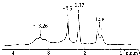
Fig. 2. Nuclear Magnetic Resonance Spectrum of C_{14}H_{18}O_5 Acid, measured in Pyridine at 60 Mc.p.s.
