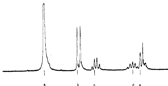
Fig. 1.—Nuclear magnetic resonance spectrum of dibenzyl propyl phosphate.
