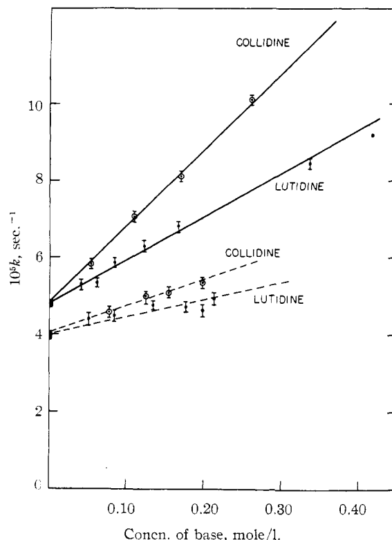
Fig. 2.—Rate of solvolysis of tetrabenzylpyrophosphate at 50°. The solid lines refer to reaction in C_3H_7OH as solvent; the dotted lines to reaction in C_3H_7OD as solvent.
