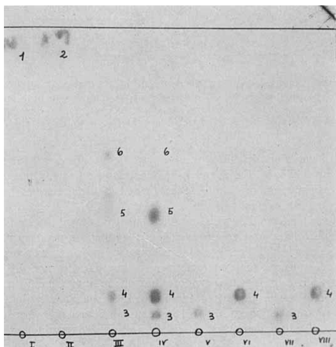
FIG. 3. Thin-layer autoradiograph of the synthesis of L- ^{14}\text{C} -serine-labelled L-SEP and L-SSP.
