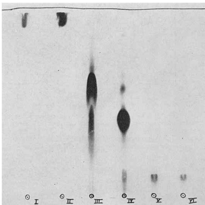
FIG. 4. Thin-layer autoradiograph of the synthesis of L- ^{14}\text{C} -threonine-labelled L-TEP.
