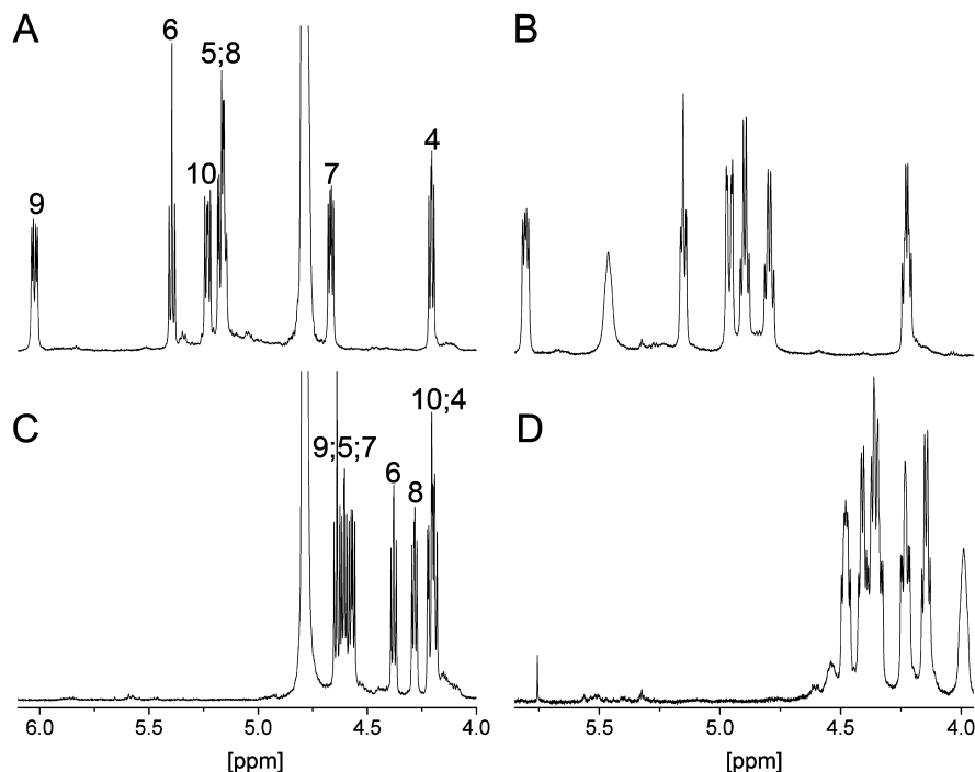
Figure 3. H^{\alpha} regions of ^1H NMR spectra of peptide 28 (A and B) and MT-II (C and D). Spectra A and C were detected in 50 mM sodium acetate- d_4 D_2O buffer (pH 4.5), B and D were detected in DMSO-d_6 . Numbers refer to H^{\alpha} atoms of the respective residues in the \alpha -MSH sequence.
