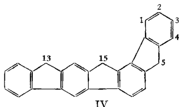
IV dihydro-13, 15-5 H -bis-indéno- [1, 2- a ; 1', 2'- h ]fluorène
