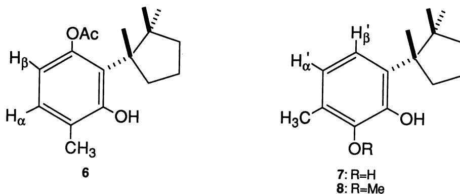
Fig. 2. Structures of compound 6-8.
