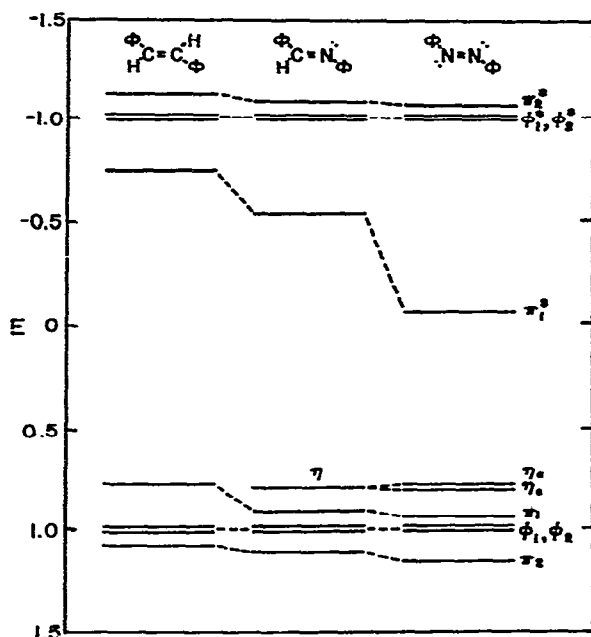
Fig. 5. One-electron orbital energy level diagrams for stilbene, benzaniline and azobenzene (from ref. 11). The LCAO orbital energy is expressed in \beta , the resonance integral for the benzene rings. In stilbene, \pi_1 is localized on the double bond as are the \eta orbitals in benzaniline and azobenzene. The \pi_1^* orbital is localized on the double bond for all three species.
