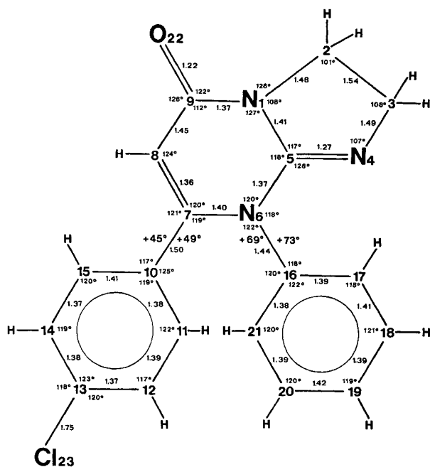
Fig. 2. Bond lengths, bond angles and some torsion angles. Standard deviations are \sigma(\text{bond}) \approx 0.015 \text{ \AA} , \sigma(\text{angles}) \approx 1.2^\circ , \sigma(\text{torsion angles}) \approx 1.6^\circ .
