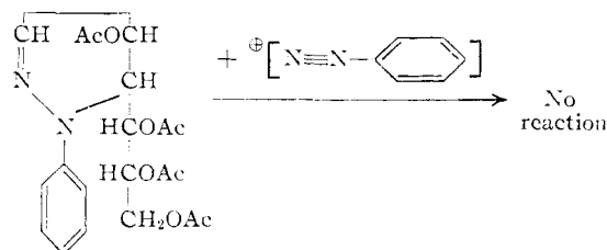
Anhydro-D-mannose phenylhydrazone tetraacetate
