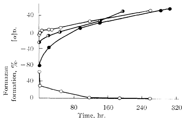
Fig. 4.—Upper curves, mutarotation of D-glucose phenylhydrazones ( c 5.4, pyridine-ethanol (1:1 by vol.)); ●, "α"-D-glucose phenylhydrazone; ○, Skraup's D-glucose phenylhydrazone; ○, "β"-D-glucose phenylhydrazone. Lower curve, D-glucose diphenylformazan formation in a mutarotating solution of aldehyde -D-glucose phenylhydrazone. No formazan was produced by the cyclic D-glucose phenylhydrazones during mutarotation.
