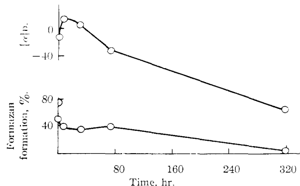
Fig. 2.—Upper curve, mutarotation of L-rhamnose phenylhydrazone ( c 1.27, pyridine-ethanol (1:1 by vol.)); lower curve, L-rhamnose diphenylformazan formation.
