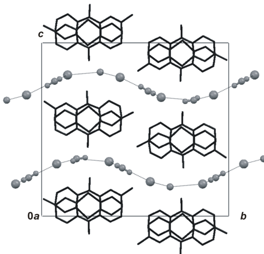
Figure 5. The packing of monosalts (3) and (4) in the crystal. H-bonds between water molecules and \Gamma^- anions are shown with dotted lines.
