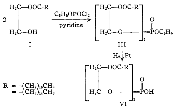
bis-(glycol)-phosphatidic acid REACTION SCHEME II
