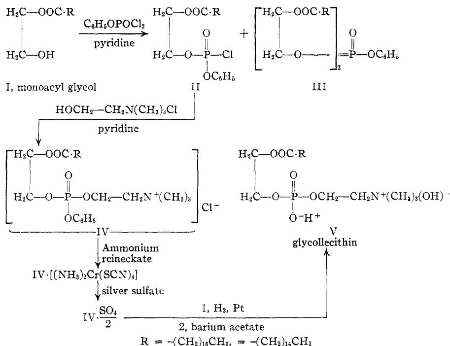
REACTION SCHEME I
