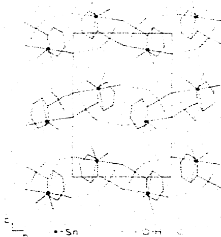
Fig. 2. Projection of the unit cell on to the bc plane showing the chains of hydrogen-bonded molecules. Hydrogen bonds are shown by dotted lines.
