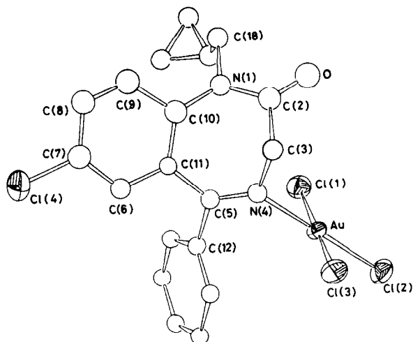
Fig. 2. ORTEP view of compound IIa , (Prazepam) \text{AuCl}_3 . The hydrogen atoms have been omitted for clarity.
