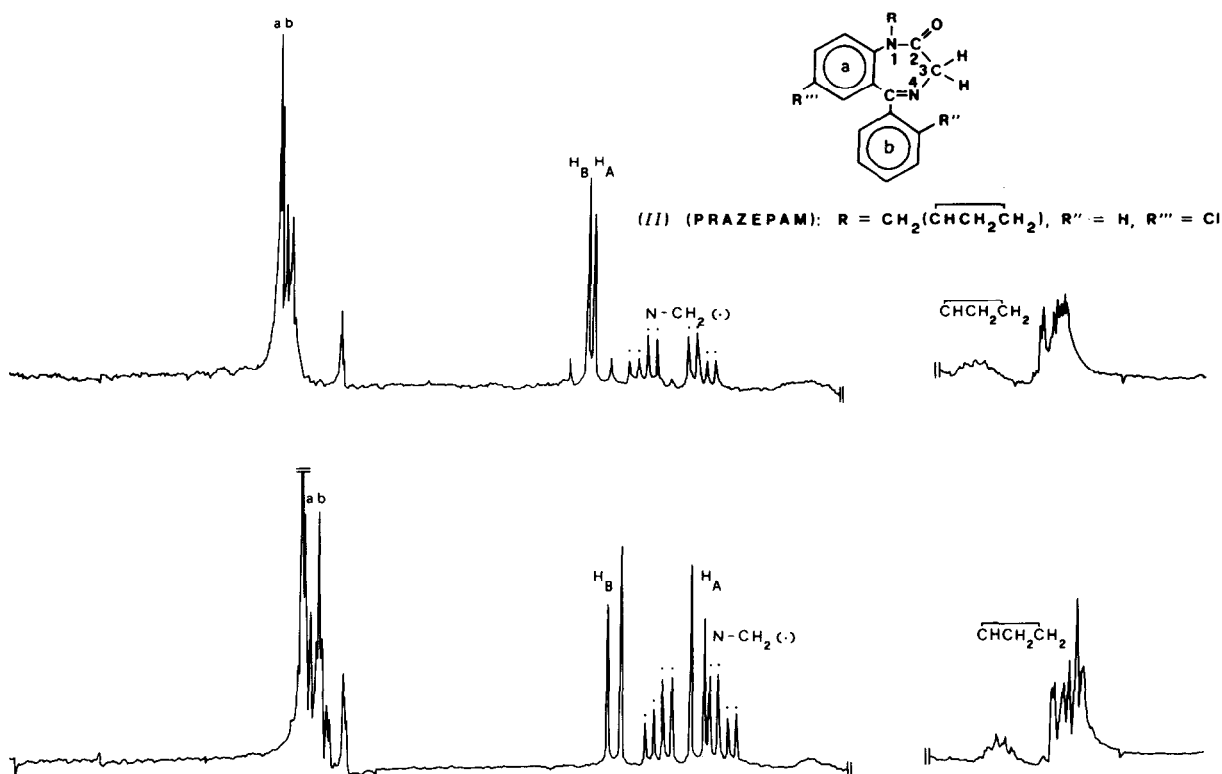
Fig. 1. ^1\text{H} NMR in deuterioacetone at room temperature. Top: compound IIa , (Prazepam) \text{AuCl}_3 ; bottom: ligand II , Prazepam.
