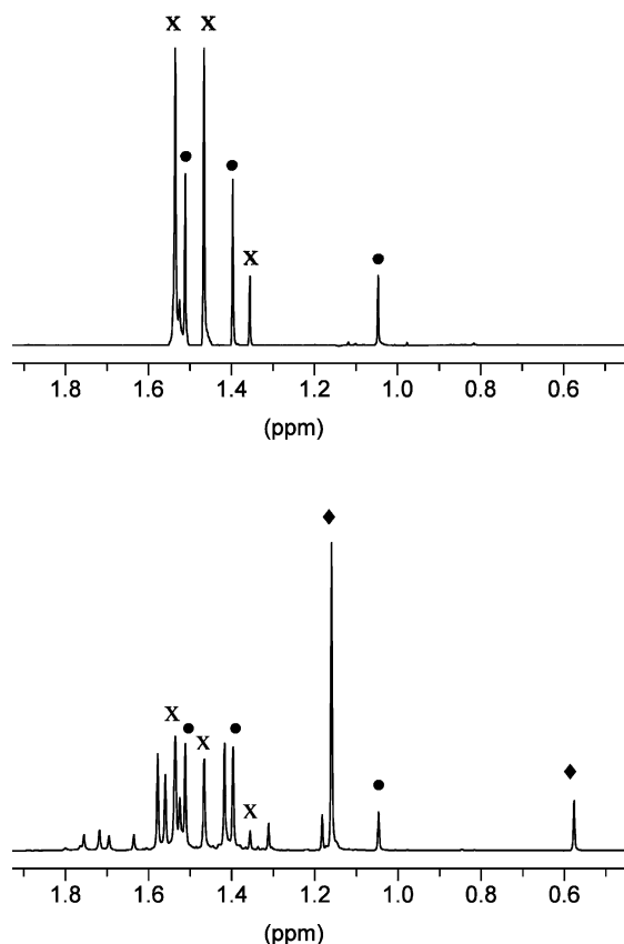
Fig. 1. ^1\text{H} -NMR spectra of 1 ( \times ) and 2 ( \bullet ) in \text{C}_6\text{D}_6 ; above: a fresh sample; below: sample after 1 day at room temperature with formation of ^t\text{Bu}_2\text{SbMe} ( \blacklozenge ) and other products.
