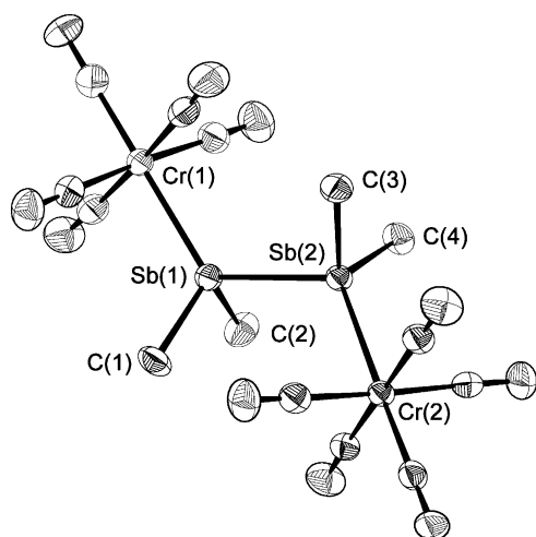
Fig. 2. ORTEP-like representation at 50% probability of 6 showing the atomic numbering scheme. Selected distances (Å) and angles ( ^\circ ): Sb(1)–Sb(2) 2.8097(9), Sb(1)–C(1) 2.132(4), Sb(1)–C(2) 2.150(4), Sb(2)–C(3) 2.141(3), Sb(2)–C(4) 2.135(3), Sb(1)–Cr(1) 2.629(9), Sb(2)–Cr(2) 2.621(8), C(1)–Sb(1)–C(2) 99.20(18), C(3)–Sb(2)–C(4) 100.34(16), Cr(1)–Sb(1)–Sb(2) 122.39(3), Cr(2)–Sb(2)–Sb(1) 118.33(2).
