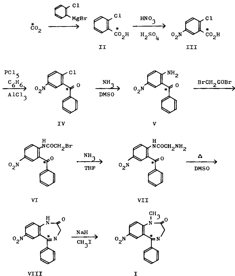
Fig. 1. Reaction Sequence of Synthesis of Nimetazepam-5- ^{14}\text{C}
