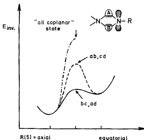
Fig. 3. Energy profile for different inversion processes in the reduced flavin (cf. Fig. 1):
