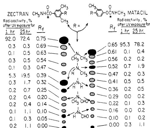
Figure 2. Photodecomposition products of Zectran-carbonyl- C^{14} and Matacil-carbonyl- C^{14} resulting from exposure on TLC plates to short-wavelength ultraviolet light
