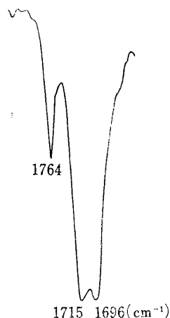
Fig. 1. Infrared Spectrum of Itaconitin p -Nitrophenylhydrazide (KBr)
