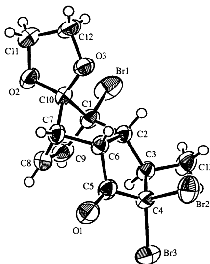
Fig. 1. ORTEP (Johnson, 1976) drawing of (II). Displacement ellipsoids are drawn at the 50% probability level. H atoms are given arbitrary radii of 0.1 Å.
