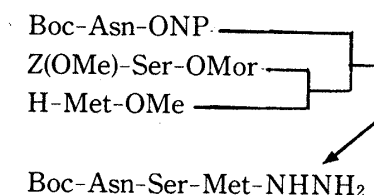
Fig. 3. Synthetic Scheme for the Protected Tripeptide Hydrazide, [5] Boc-(hPTH 16—18)-NHNH 2
