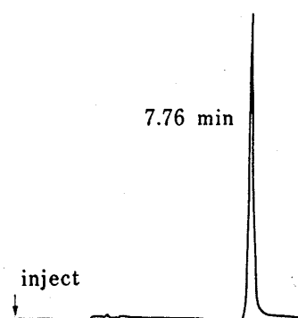
Fig. 7. HPLC of Synthetic H-(hPTH 1-34)-NH 2
