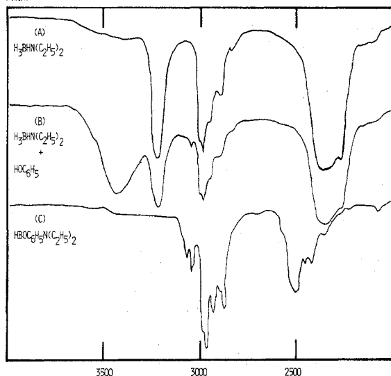
Figure 1. Infrared spectra (4000-2000 \text{cm}^{-1} ) of diethylamine-borane (A), an equimolar mixture of phenol and diethylamine-borane (B), and diethylaminohydridophenoxyborane (C).
