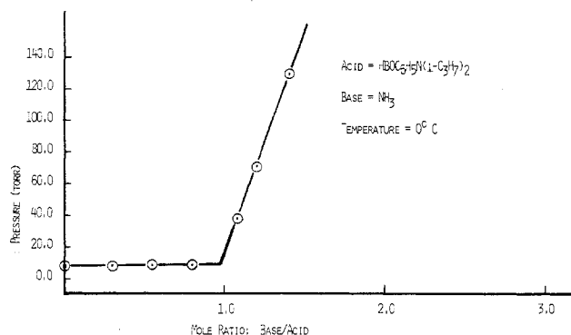
Figure 4. Tensimetric titration of diisopropylaminohydridophenoxyborane with ammonia.
