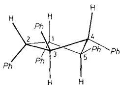
Abb. 2. Pentaphenylcyclopentasilan
