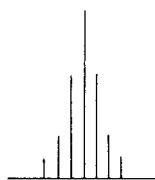
Figure 3. ESR spectrum of IVc in CH_2Cl_2 solution at room temperature.
