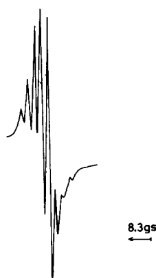
Figure 1. ESR spectrum of IVa in THF solution at room temperature.
