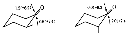
Figure 4. Enthalpy interactions of a 2-methyl group to reduction by NaBH 4 , over and above those existing in cyclohexanone (figures in parentheses).
