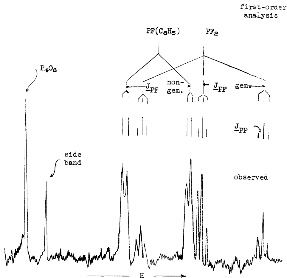
Figure 1.—Phosphorus-31 nuclear magnetic resonance spectrum of trans -1,3- \text{P}_3\text{N}_3\text{F}_4(\text{C}_6\text{H}_5)_2 . Scale = 228.4 \text{ Hz cm}^{-1} .
