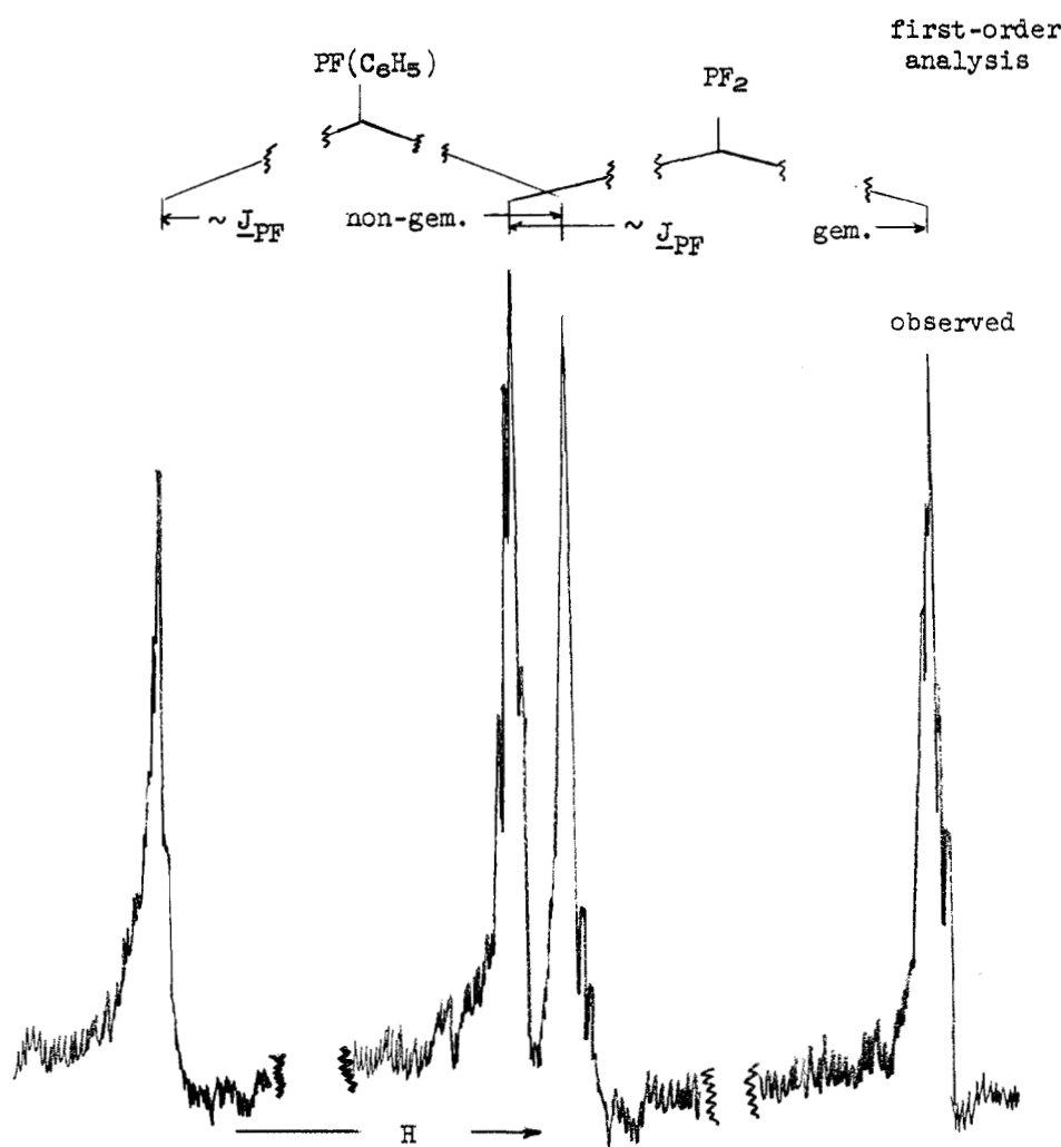
Figure 3.—Fluorine-19 nuclear magnetic resonance spectrum of trans -1,3- N_3P_3F_4(C_6H_5)_2 . Scale = 100 Hz cm^{-1} .
