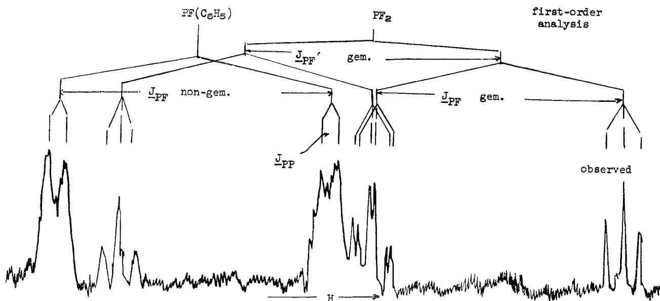
Figure 2.—Phosphorus-31 nuclear magnetic resonance spectrum of cis - \text{N}_3\text{P}_3\text{F}_4(\text{C}_6\text{H}_5)_2 . Scale = 106.4 \text{ Hz cm}^{-1} .
