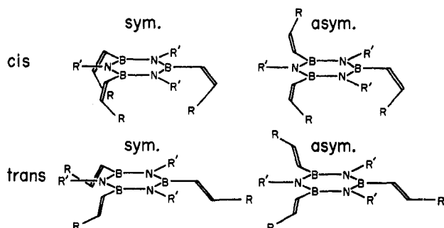
Figure 1.—Structures of B-trivinylborazine derivative.
