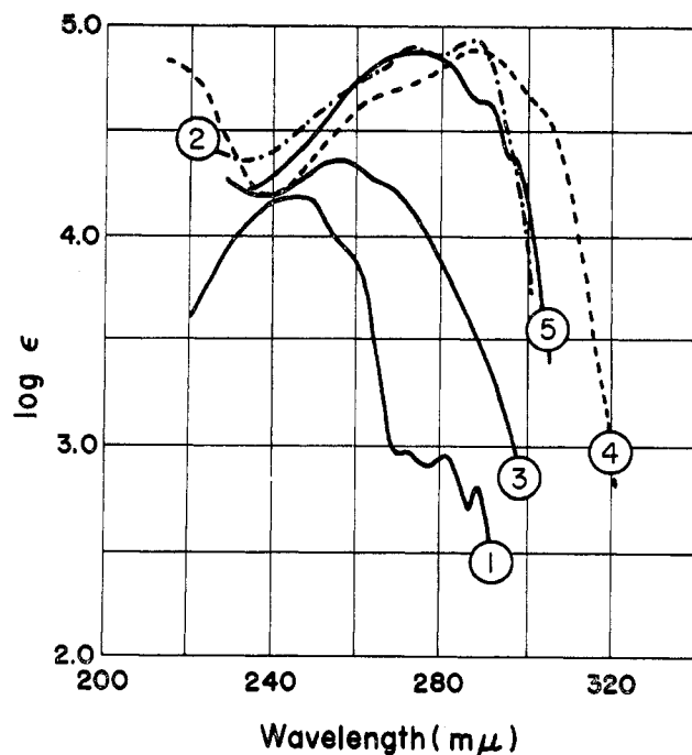
Figure 2.—Ultraviolet spectra of 1, styrene; 2, B_3(C\equiv C-C_6H_5)_3N_3(C_6H_5)_3 ; 3, B_3(cis-CH=CH-C_6H_5)_3N_3(C_6H_5)_3 (VI); 4, B_3(trans-CH=CH-C_6H_5)_3N_3(C_6H_5)_3 (VII); and 5, B_3(cis-CH=CH-C_6H_5)_3N_3H_3 (II).
