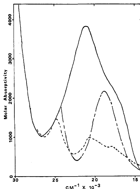
Figure 5.—Electronic absorption spectra of [\text{Ni}(\text{C}_{32}\text{H}_{34}\text{N}_2\text{P}_2)\text{Br}]\cdot\text{ClO}_4\cdot 0.5\text{C}_2\text{H}_5\text{OH} (—), [\text{Ni}\{\text{Ph}_2\text{P}(o\text{-C}_6\text{H}_4\text{AsPPh}_2)\}_2\text{Br}]\cdot\text{ClO}_4 (---), and \text{Ni}\{\text{CH}_3\text{As}(\text{CH}_2\text{CH}_2\text{CH}_2\text{AsMe}_2)_2\}\text{Br}_2 (- - -) in dichloromethane solution.
