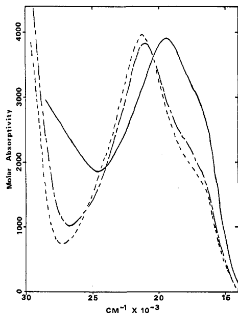
Figure 3.—Electronic absorption spectra of [\text{Ni}(\text{C}_{32}\text{H}_{34}\text{N}_2\text{P}_2)\text{I}]\cdot\text{ClO}_4\cdot 0.5\text{C}_2\text{H}_5\text{OH} (—), [\text{Ni}(\text{C}_{32}\text{H}_{34}\text{N}_2\text{P}_2)\text{Br}]\cdot\text{ClO}_4\cdot 0.5\text{C}_2\text{H}_5\text{OH} (---), and [\text{Ni}(\text{C}_{32}\text{H}_{34}\text{N}_2\text{P}_2)\text{Cl}]\cdot\text{ClO}_4\cdot 0.5\text{C}_2\text{H}_5\text{OH} (- - -) in dichloromethane solution.
