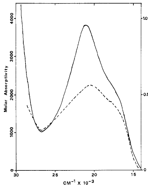
Figure 2.—Electronic absorption spectra of [Ni(C 32 H 34 N 2 P 2 )Br]ClO 4 ·0.5C 2 H 5 OH in the solid state (----) and in dichloromethane solution (—).
