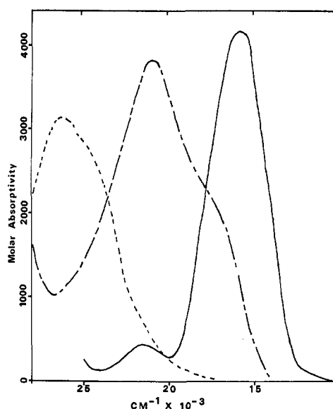
Figure 4.—Electronic absorption spectra of [\text{NiAs}(o\text{-C}_6\text{H}_4\text{AsPh}_2)_3\text{Br}]\cdot\text{ClO}_4 (—), [\text{Ni}(\text{C}_{32}\text{H}_{34}\text{N}_2\text{P}_2)\text{Br}]\cdot\text{ClO}_4\cdot 0.5\text{C}_2\text{H}_5\text{OH} (---), and [\text{Ni}(\text{C}_{32}\text{H}_{34}\text{N}_2\text{P}_2)](\text{ClO}_4)_2 (- - -) in dichloromethane solution.
