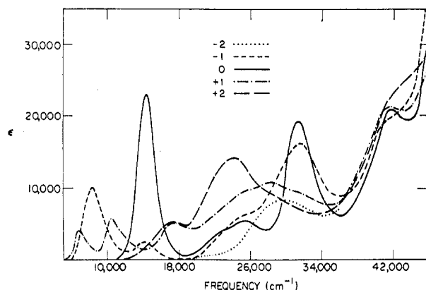
Figure 2.—Electronic absorption spectra of Pt(C 6 H 5 , tert -C 4 H 9 -atf) 2 z species. The z = 1- , 1+ , 2+ ions were generated by controlled-potential electrolysis of acetonitrile solutions of z = 0 , and the z = 2- ion was produced by sodium amalgam reduction of z = 0 in THF. The band at 14,400 cm -1 in the spectrum of the monoanion arises from incomplete reduction of the neutral complex.
