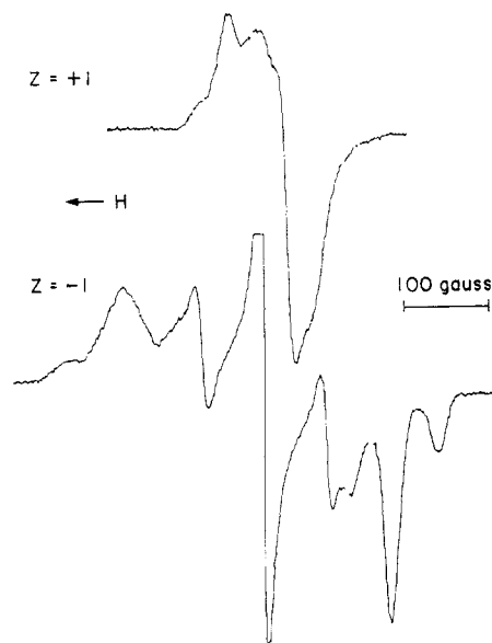
Figure 3.—Epr spectra of Pt(C 6 H 5 ,(CH 3 ) 2 -atf) 2 z species in glasses at ~-196°: upper, z = 1+ produced by oxidation of z = 0 with bromine in CHCl 3 -DMF; lower, z = 1- generated by reduction of z = 0 with sodium amalgam in 2-CH 3 THF.
