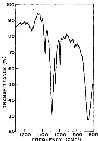
Fig. 1. The infrared spectrum ( 1250-800\text{ cm}^{-1} ) of a Nujol dispersion of C_6H_5SO_2HgC_6H_5 [isomer (I)].
