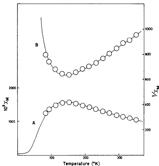
Figure 2. The temperature dependence of 10^6 \chi_M (A), and 1/\chi_M (B) for \text{Cu}_2(3\text{MeOONMeS})\text{Cl}_3 . Experimental values are indicated by open circles and the full curves are the calculated values obtained from the Bleaney-Bowers equation (1) with g = 2.13 and J = -79 \text{ cm}^{-1} .
