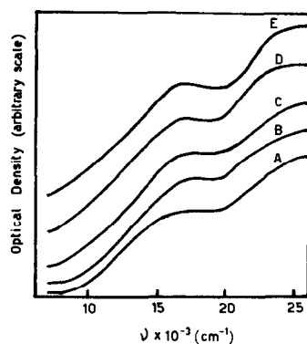
Figure 1. Solid state reflectance spectra of copper complexes: A, [\text{Cu}(\text{ONMeS})\text{py}]\text{ClO}_4 ; B, \text{Cu}_2(\text{ONMeS})_2\text{Cl}_4 ; C, \text{Cu}_2(\text{ONMeS})_2\text{Cl}_4 ; D, \text{Cu}(\text{ONMeS})\text{NO}_3 ; E, \text{Cu}(\text{ONMeS})\text{NO}_3 .
