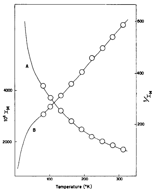
Figure 3. The temperature dependence of 10^6 \chi_M (A) and 1/\chi_M (B) for \text{Cu}_3(\text{ONSMe})_2\text{Cl}_4 . Experimental values are indicated by open circles and the full curves are the calculated values obtained from equation (3) for a linear trimer structure, with g = 2.48 and J = -37 \text{ cm}^{-1} .
