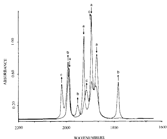
Fig. 4. Infrared spectral changes upon photolysis of complex 1 with \lambda = 630 nm ( P = 35 mW) in THF at 293 K: (a) 1 ; (b) \text{Cp}_2\text{Fe}_2(\text{CO})_4 ; (c) \text{Re}(\text{CO})_3(\text{bpy}') .
