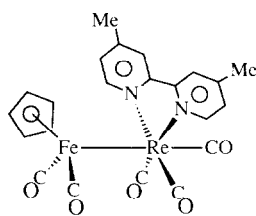
Fig. 1. Proposed structure of \text{CpFe(CO)}_2\text{Re(CO)}_3(\text{bpy}') .
