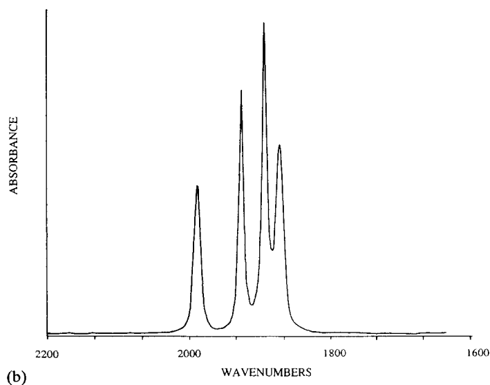
Fig. 2. (a) UV-Vis and (b) infrared (CO-stretching region) spectrum of \text{CpFe(CO)}_2\text{Re(CO)}_3(\text{bpy}') (1) at 293 K in THF.
