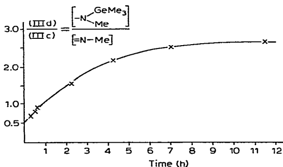
Fig. 1. Variation of the ratio [\text{III d}]/[\text{III c}] during the reaction of \text{Me}_3\text{Si-NMe-GeMe}_3 with \text{Ph-N}=\text{C}=\text{O} in \text{CCl}_4 at 25^\circ .
