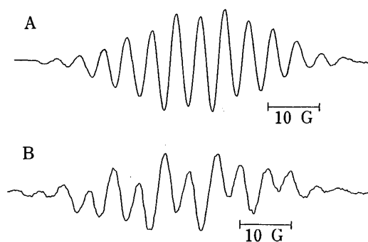
Fig. 3. ESR Spectra of in Situ Electrolyzed Solutions of the Sulfenamidides 3 (10 mM) at 25 °C (A) and 4 (10 mM) at -40 °C
