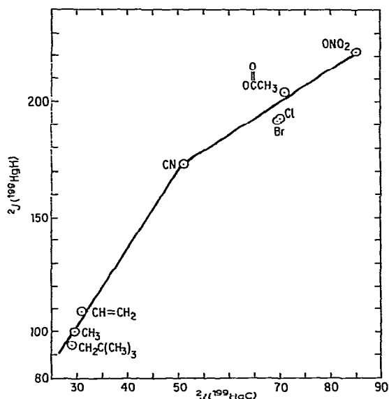
Fig. 3. Plot of ^2J(^{199}\text{HgH}) vs. ^2J(^{199}\text{HgC}) of (\text{CH}_3)_3\text{CCH}_2\text{Hg-R (or X)} .
