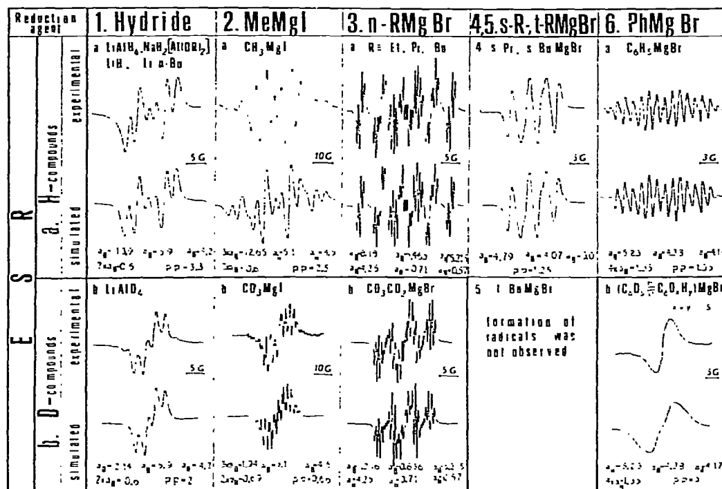
Fig. 1. Experimental and simulated ESR spectra of radicals formed by the reaction of nucleophilic disopropylsilylate with different deuterated and non-deuterated reagents ( a_H , a_D are the coupling constants, pp the peak-to-peak widths of the simulated spectra, expressed in Gauss).
