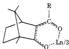
I \text{Ln}(\text{facam})_3 , \text{R} = \text{CF}_3 \text{Ln}(\text{hfbc})_3 , \text{R} = \text{C}_3\text{F}_7
