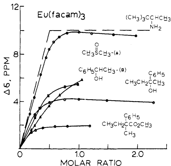
Figure 4. Plots of \Delta\delta vs. molar ratio for the designated protons of the various compounds in the presence of 0.3 M \text{Eu}(\text{facam})_3 . The intersecting dashed lines represent a hypothetical case involving the formation of a 1:2 reagent-substrate complex assuming no dissociation and a chemical shift of 10 ppm for the complex.
