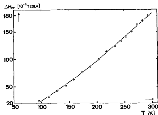
Fig. 9. Temperature-dependence of the ESR. line-width for \text{Ni}(\text{dtdbtaa})\text{I}_{2.58} crystals
