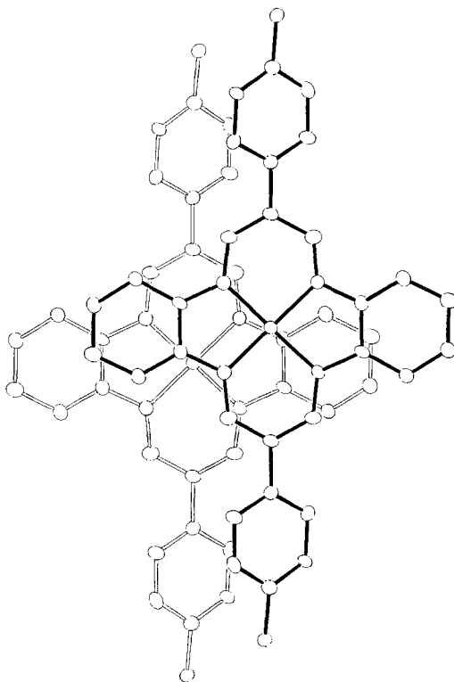
Fig. 8. Overlap of two neighbouring molecules of a stack in Ni(dtdbtaa)I_{2.58}
