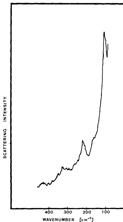
Fig. 1. Resonance-Raman spectrum of a solid sample of Ni(dtdbtaa)I 2.58 (spinning KBr disc, \nu_0 = 4880 Å; I_3^- -symmetric stretching fundamental at 106 cm -1 and overtone progression)
