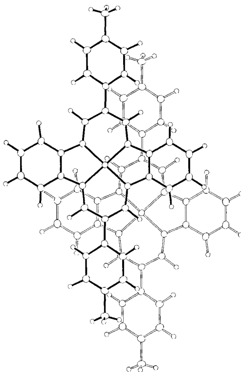
Fig. 5. Overlap of two adjacent molecules in Ni(dtdtaa) crystals
