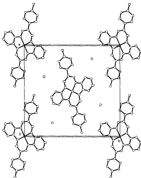
Fig. 6. Projection of the \text{Ni}(\text{dtbbta})\text{I}_{2.58} structure on the a,b-plane
