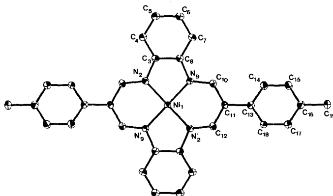
Fig. 2. Atom-labeling scheme for the macrocyclic molecule (elipsoids for all drawings are at 20% probability)
