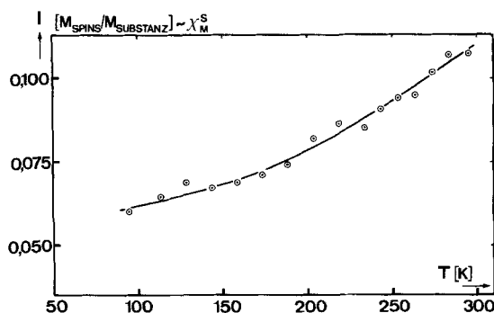
Fig. 10. Temperature-dependence of the ESR.-signal intensity (proportional to the molar spin susceptibility \chi_m^S ) in number of free spin per macrocycle for crystals of \text{Ni}(\text{dtdbtaa})\text{I}_{2.58}
