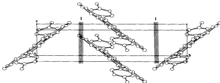
Fig. 7. Stacking of the macrocyclic molecules in \text{Ni}(\text{dtbbta})\text{I}_{2.58} illustrated in a projection on the b,c-plane
