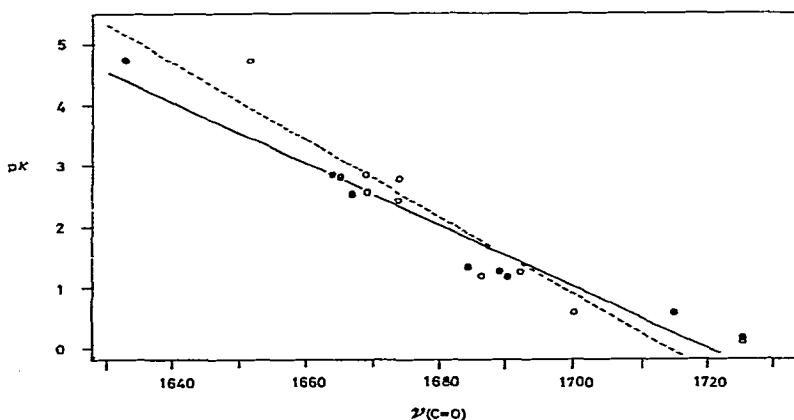
Fig. 1. The \text{pK} of the parent acid vs. the \nu(\text{C}=\text{O}) of the triphenylantimony (●) and the trimethylantimony (○) carboxylic acid derivatives.
