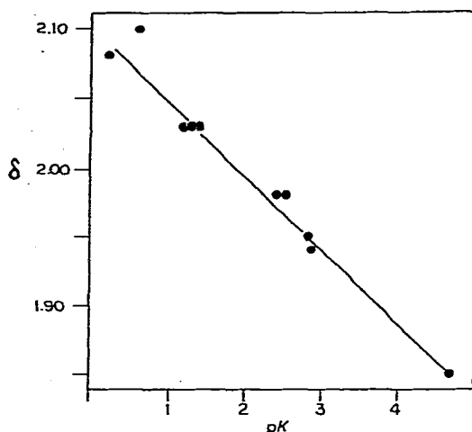
Fig. 2. Chemical shifts of \text{Me}_3\text{Sb} protons vs. the \text{pK} of the parent acid.
