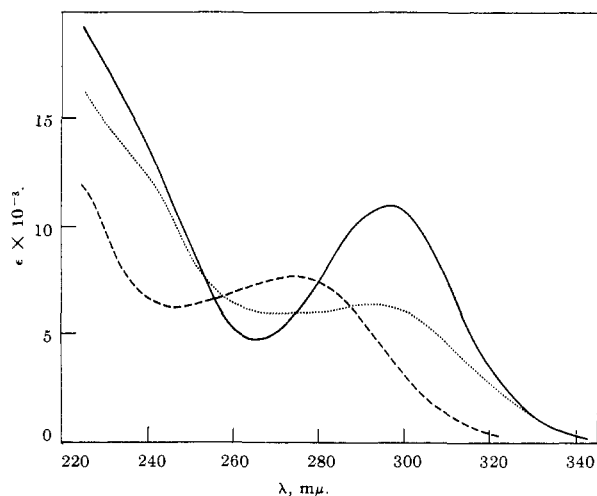
Figure 3. Ultraviolet absorption spectra of 5-( o -aminophenylthio)pyrimidine-2,4-dione: ···, neutral species; ---, monoprotated species; —, monoanionic species.
