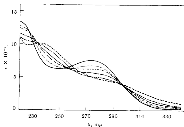
Figure 4. Ultraviolet absorption spectra of 5-( o -aminophenylthio)pyrimidine-2,4-dione in sulfuric acid solutions: —, H_0 = -2.0 ; ···, H_0 = -5.7 ; - - - -, H_0 = -6.8 ; ---, H_0 = -7.5 ; - · - · - ·, H_0 = -8.2 ; - - - - - , H_0 = -10 .
